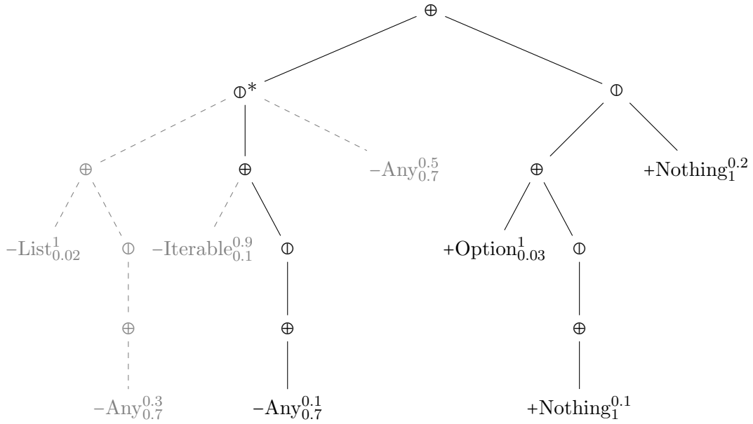
Figure 4.7.: Expression tree as shown in Figure 4.6 after applying -Iterable ; pruned nodes are shown grayed out and with dashed edges to parent nodes
