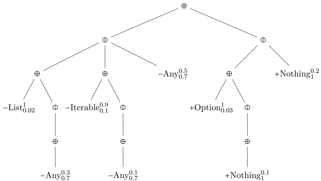
Figure 4.6.: Expression tree for the query List[T] => Option[T] ; each leaf node’s fingerprint term is annotated with the according weight (superscript) and type frequency (subscript)
