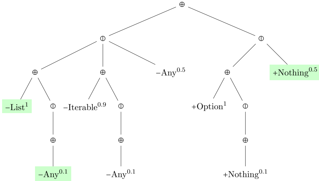
Figure 3.6.: Expression tree for the query List[T] => Option[T] marked with the fingerprint -List , -Any , -Any , +Nothing
