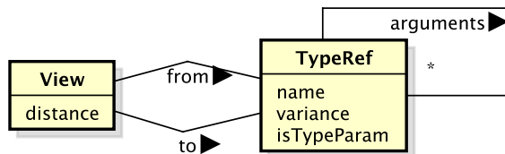
Figure 4.4.: Views as an abstraction of subtype relations
