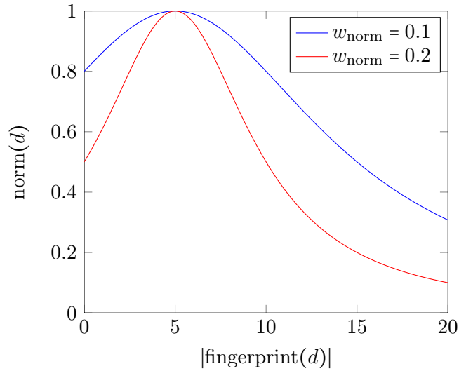
Figure 3.7.: The fingerprint length normalization function with a query fingerprint length of 5 and different values for w_{\text{norm}}
